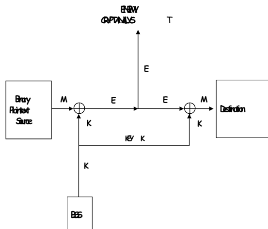
Fig. 4: Vernam’s Cipher (“Perfect Secrecy”)
