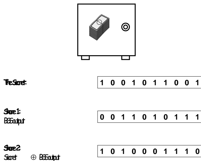
Fig. 6: “No-Leakage” Secret Sharing
